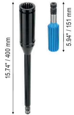
RDS 6072 AT Tata 407 N/M Heavy Duty Teflon Coated List Price Rs.1,525
