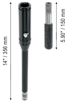
RDS 6073 Tata 609 with Grease Nipple List Price Rs.1,075
