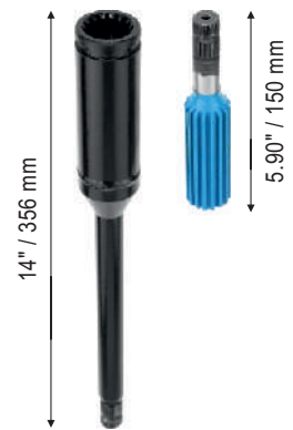
RDS 6073 AT Tata 609 Heavy Duty with Grease Nipple Teflon Coated List Price Rs.....
