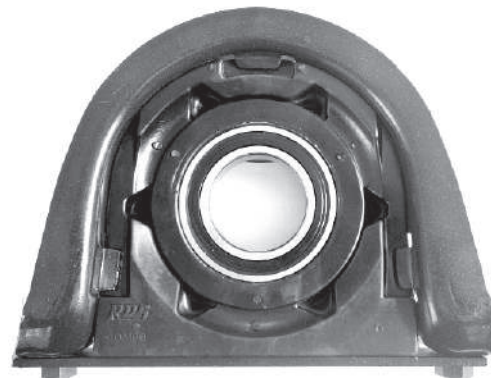
RDS 438 Tata 3718 / Bharat Benz 2523 (with 6011 - 2RS Bearing, ID 55 mm) List Price : Rs.2,260
