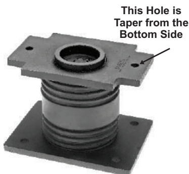
RDS HP 531 Rubber Hollow Pad Eicher BS-VI (with 12 mm Taper Holes) List Price Rs.4,400 Each
